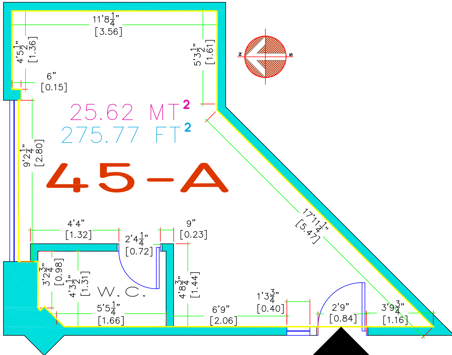
ARCHITECTURAL PLAN L-45A PLAZA "A" MEASURE'S
